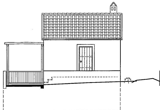
SIDE ELEVATION CDSa
