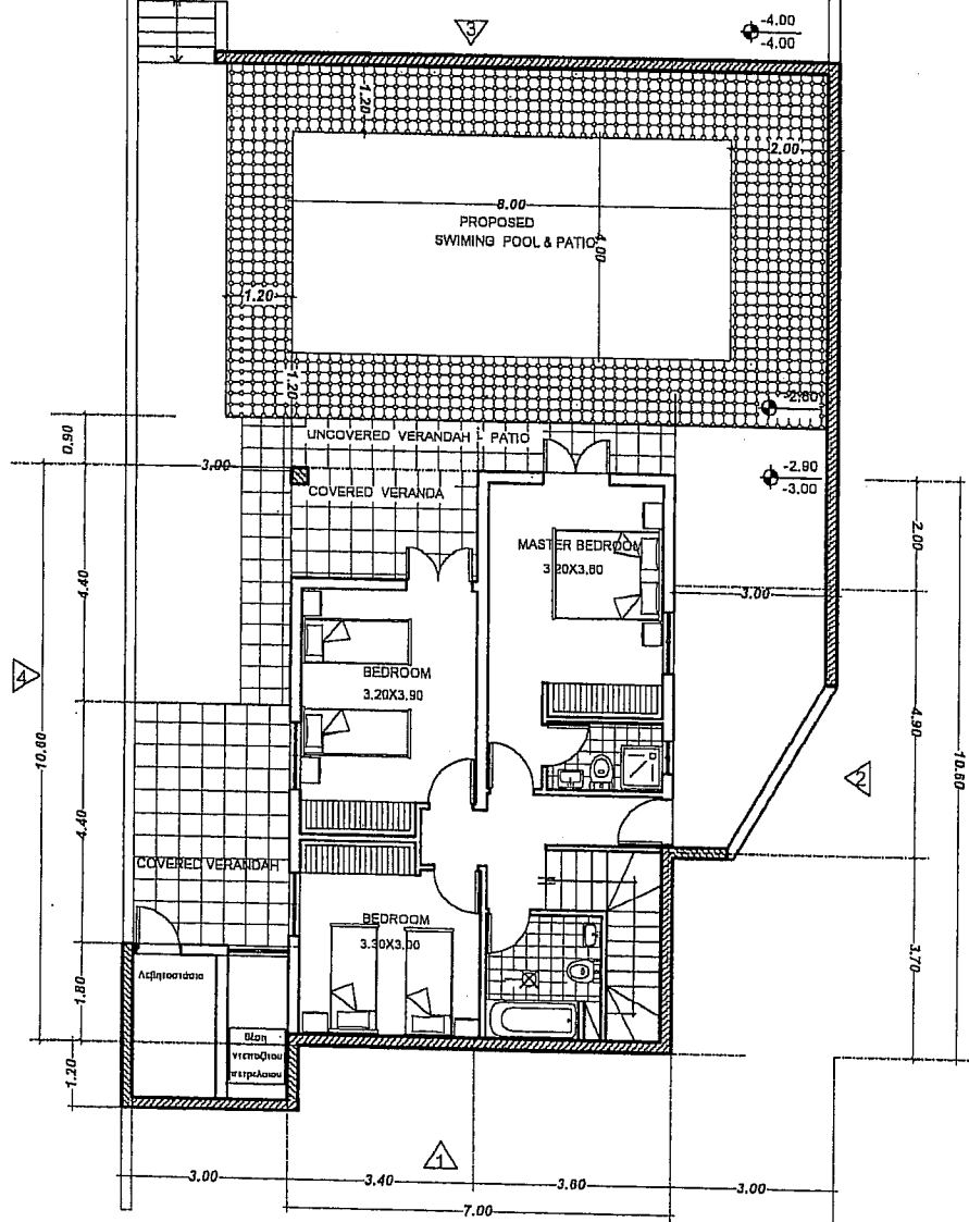
PLAN OF H5 DETACHED LOWER FLOOR 3 BEDROOM
