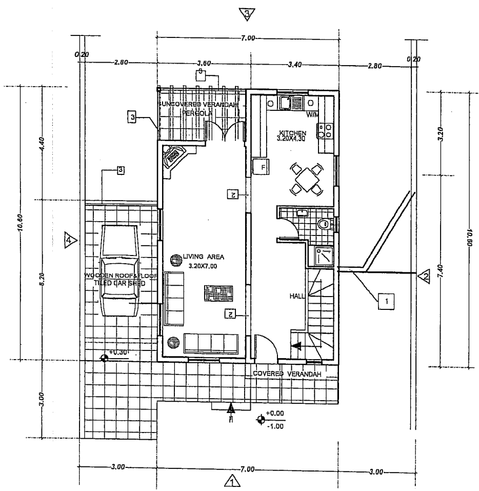
PLAN OF H5 DETACHED UPPER FLOOR 3 BEDROOM
