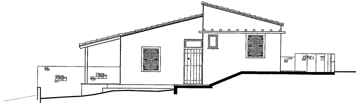
SIDE ELEVATION CB2
